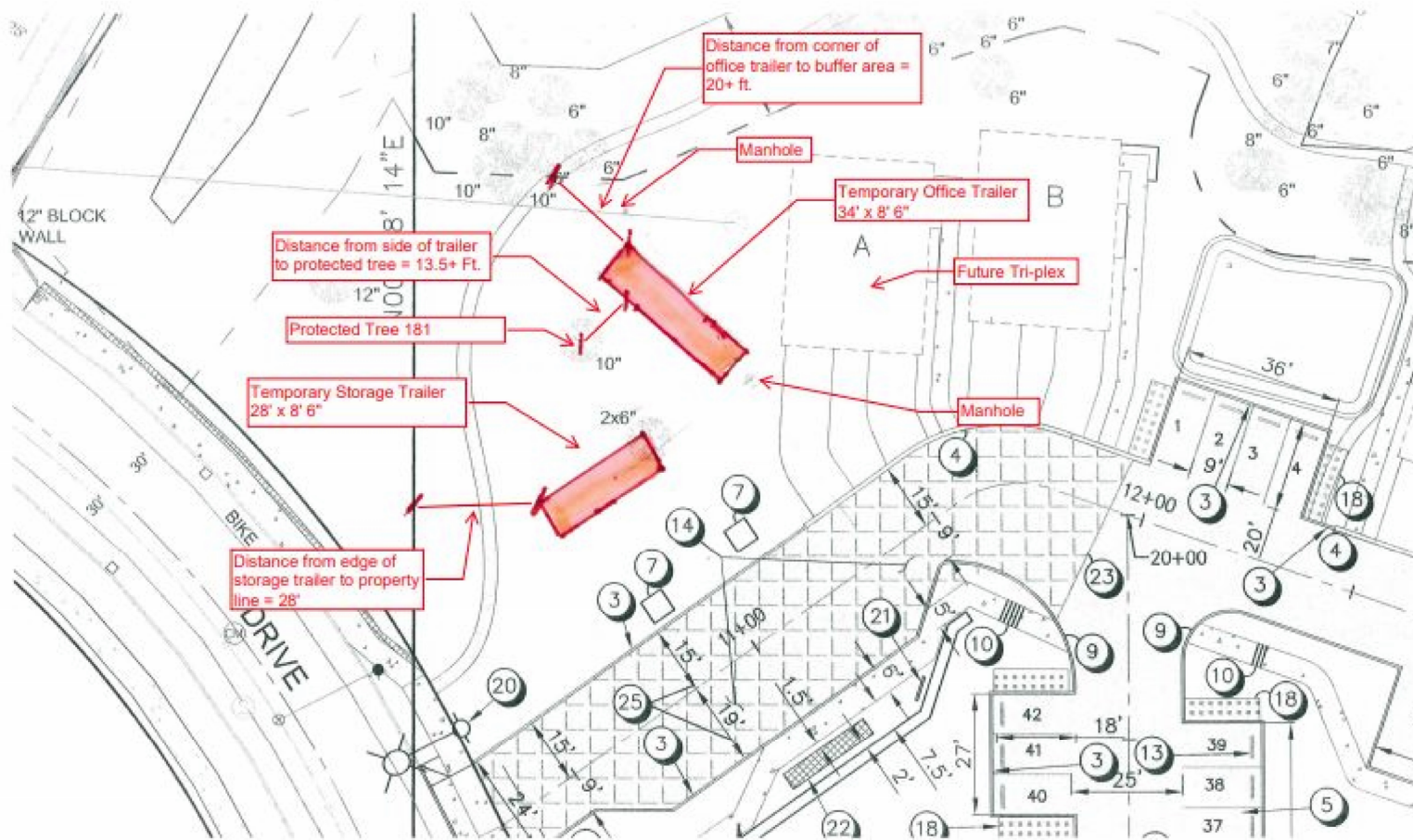
TICKLE CREEK CONSTRUCTION TRAILERS 37101 Dubarko Rd Sandy OR Scale = 1" = 30'
