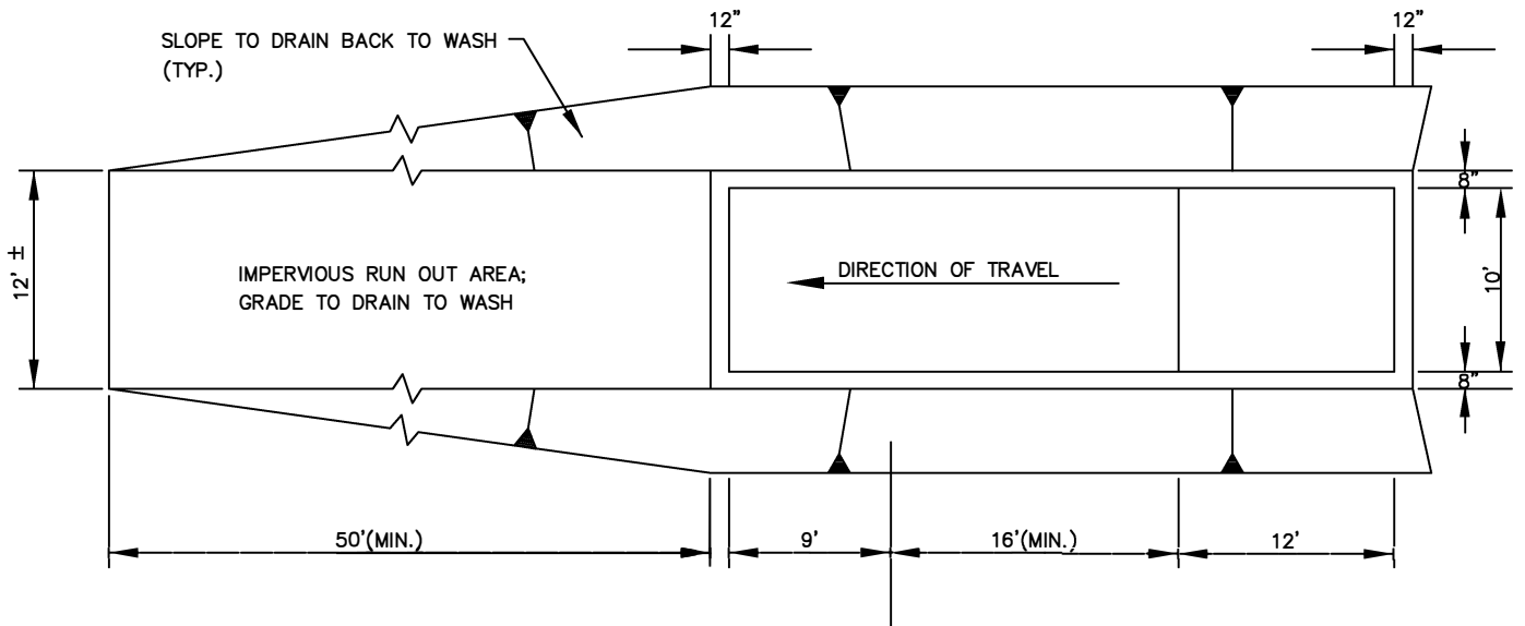
PLAN VIEW
